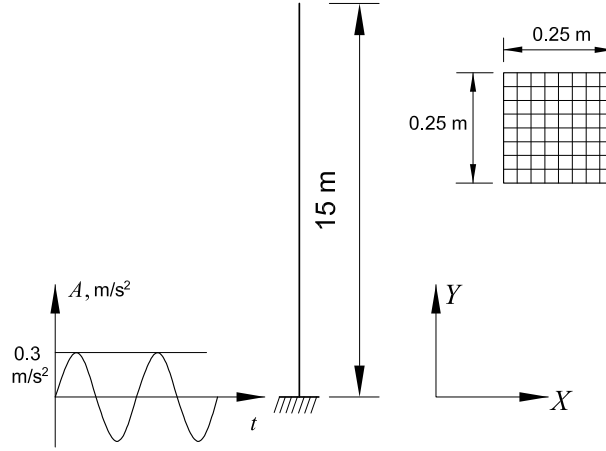
Figure 8.19: Vertical cantilever beam subjected to a sinusoidal base acceleration.
