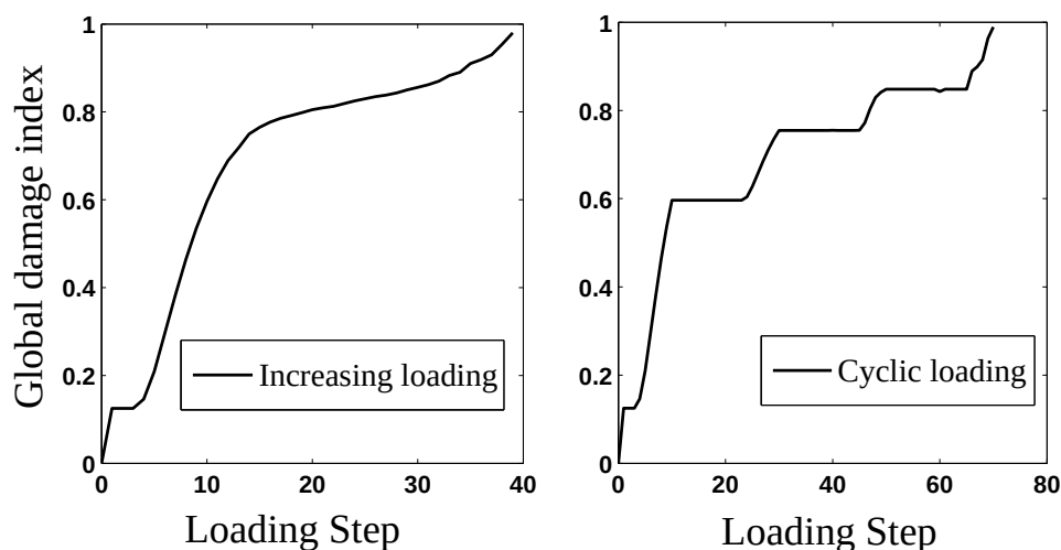
Figure 8.31: Global damage indices.
