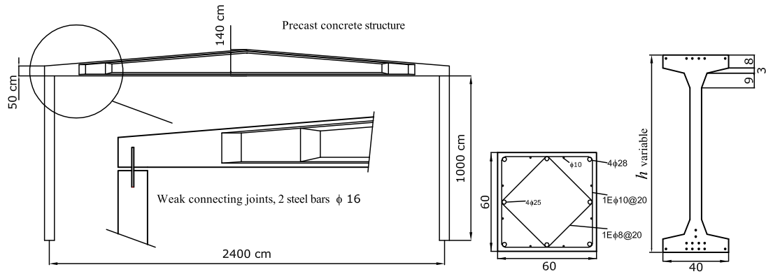
Figure 8.36: Description of the structure.
