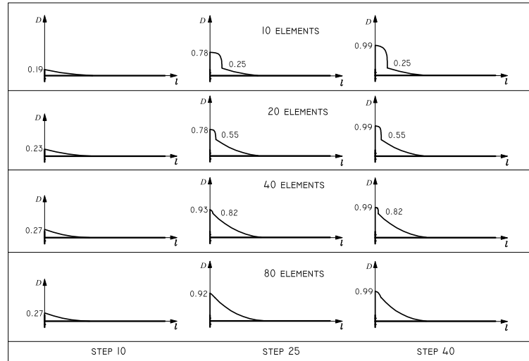
Figure 8.6: Evolution of the local cross sectional damage index: Strain localization. The symbols D and l are the damage index and the length of the beam, respectively.
