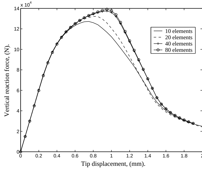
Figure 8.5: Vertical reaction versus tip displacement.
