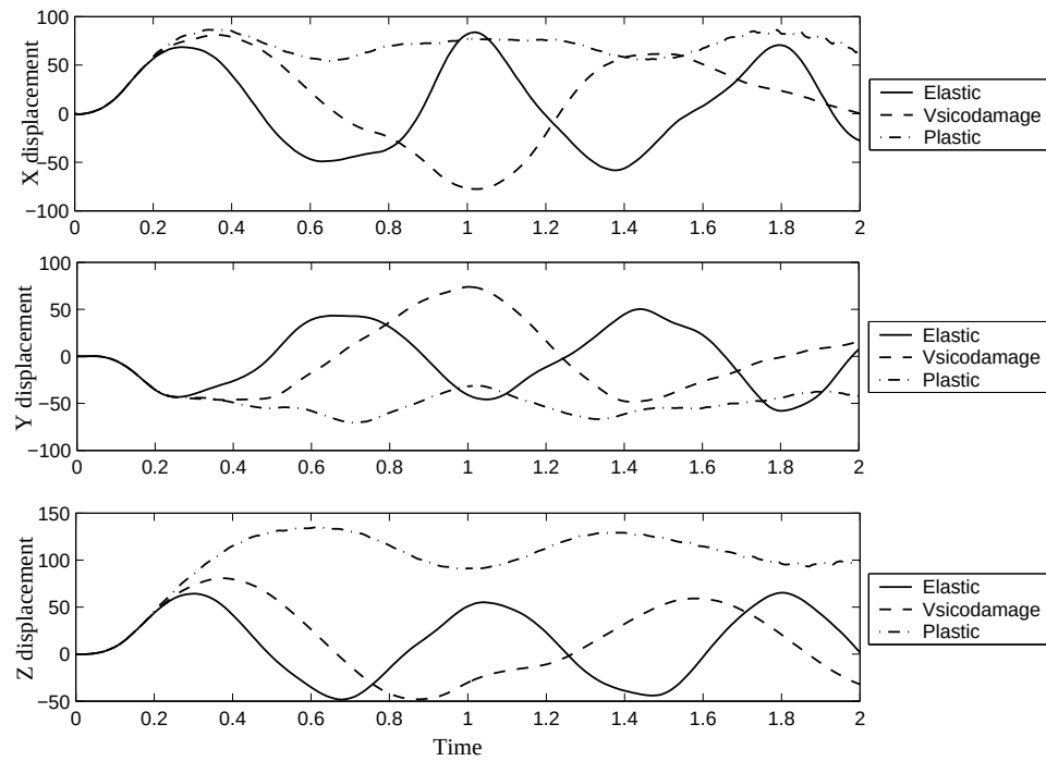
Figure 8.26: Displacement time history response of the node B.
