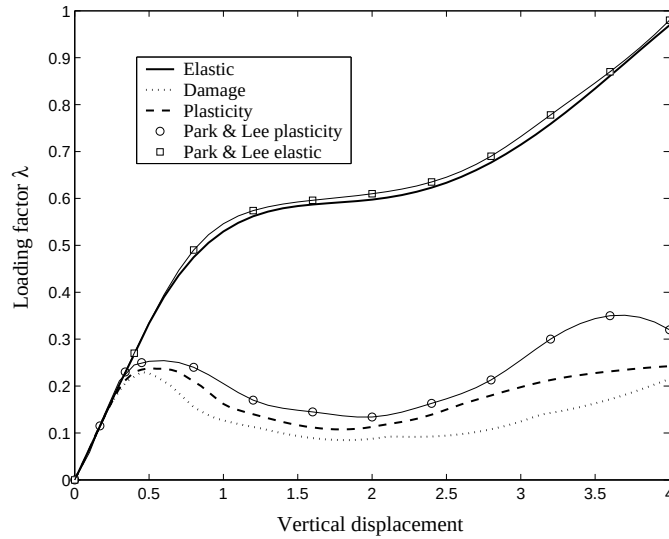
Figure 8.9: Loading factor-displacement curve of the vertical apex of the dome.
