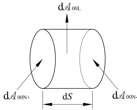
Figure 3.7: A differential slice for the straight reference configuration.
