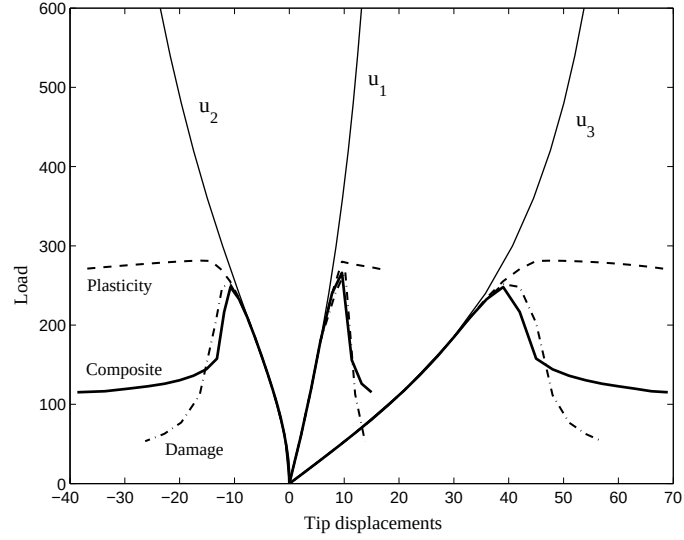
Figure 8.12: Different components of the tip displacement (nonlinear case).
