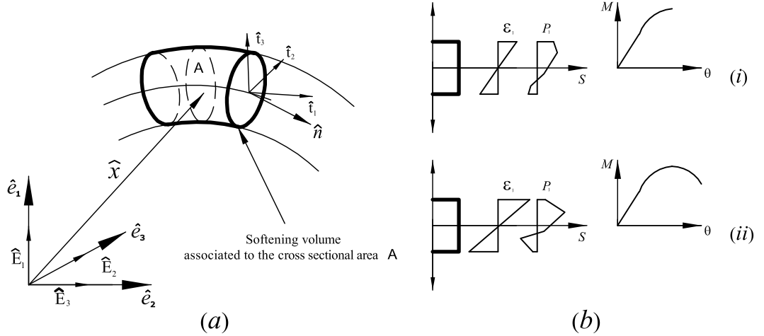
Figure 4.2: Softening volume in the rod element.
