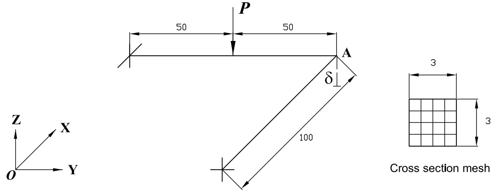
Figure 8.13: Right bent description.
