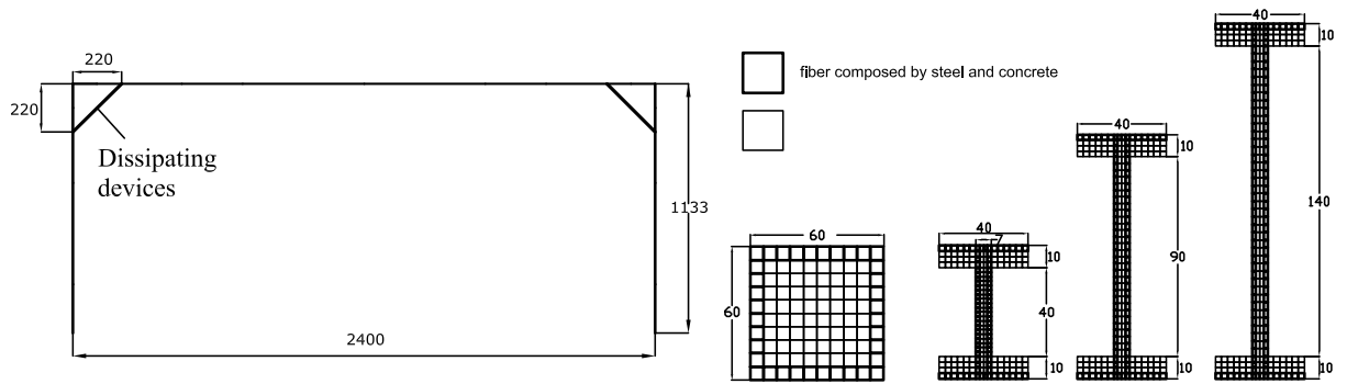
Figure 8.37: Model of the precast industrial frame with energy dissipating devices and meshes of the beam cross sections.
