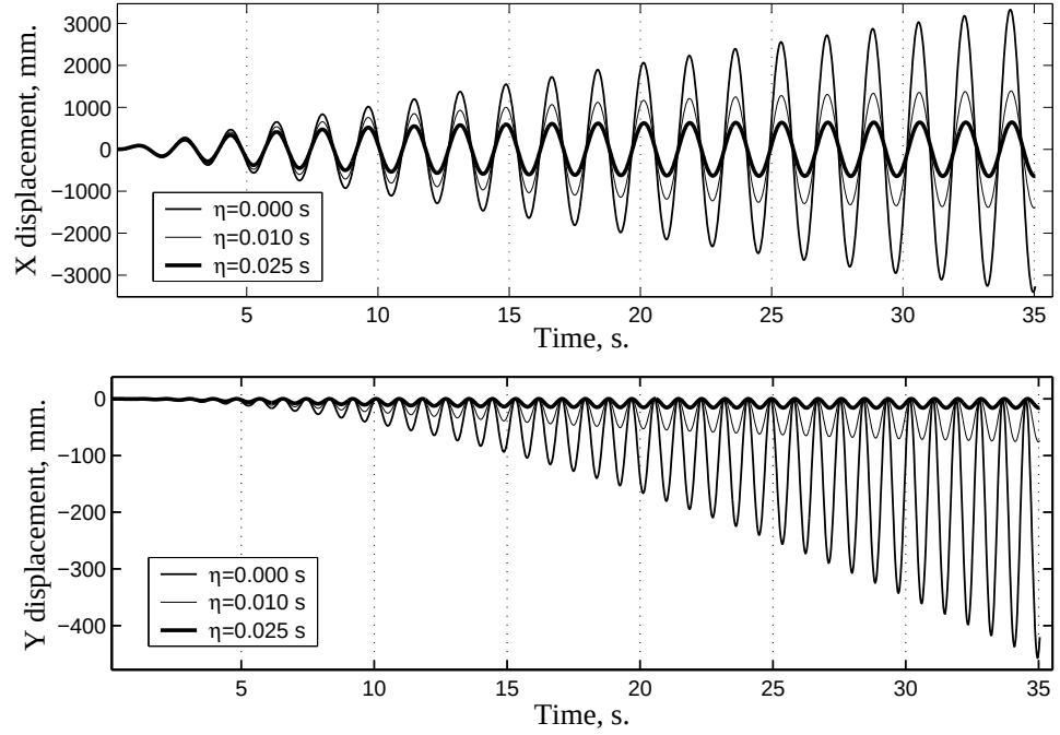
Figure 8.20: Horizontal and vertical displacement at the top.
