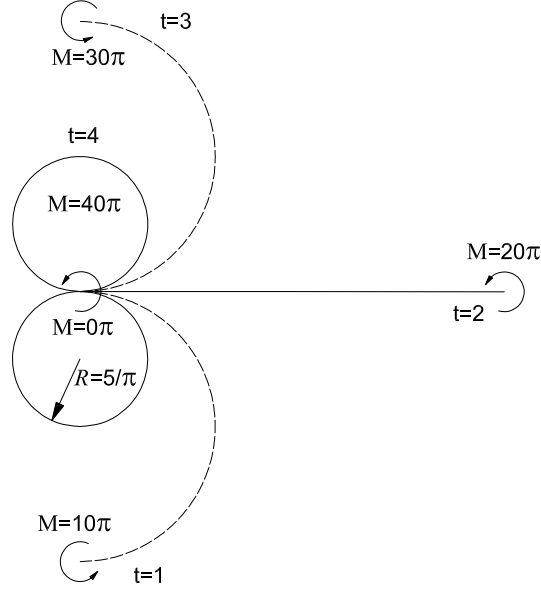
Figure 8.1: Deformed configurations of the circular beam.
