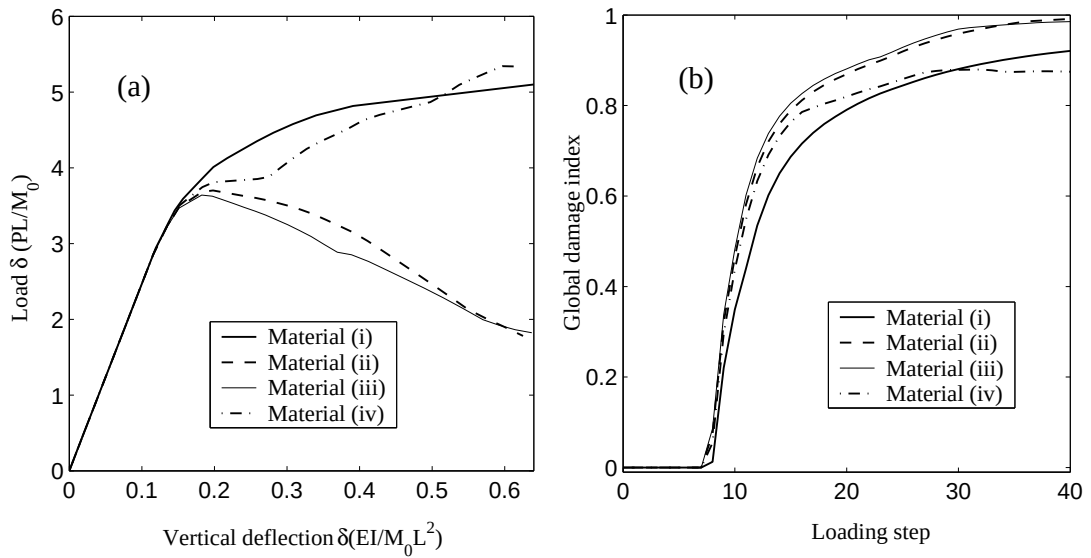
Figure 8.15: (a): Load deflection curves. (b): Global damage indices.
