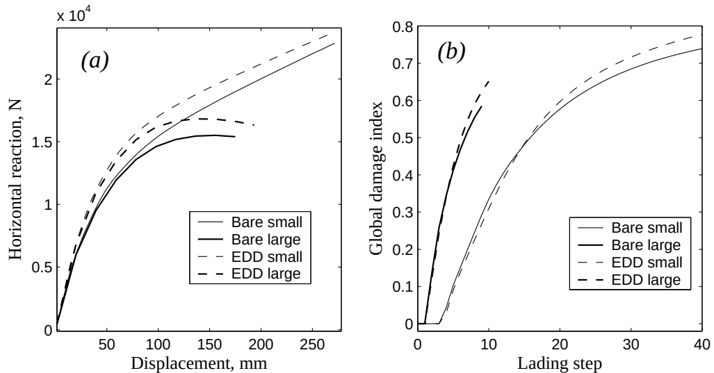
Figure 8.38: (a): Capacity curves. (b): Evolution of the global damage index.
