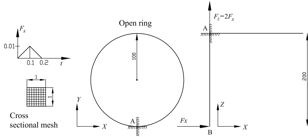
Figure 8.24: Three-dimensional curved beam structure.
