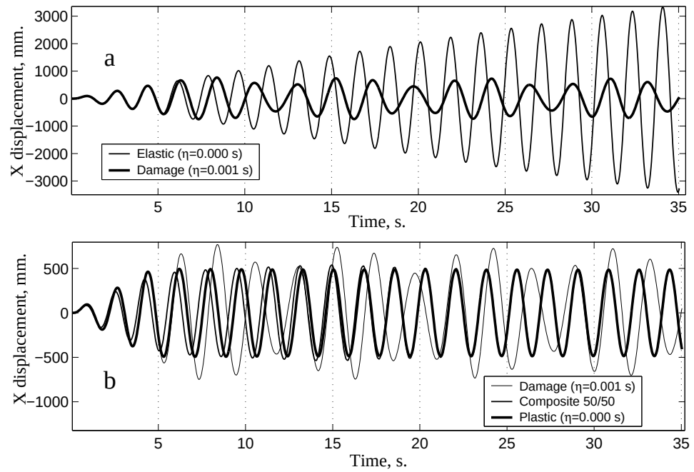
Figure 8.22: Coupled geometric and constitutive nonlinear dynamic responses. (a): Undamped elastic response compared with a visco damage constitutive model. (b): Visco damage, plastic and composite responses.
