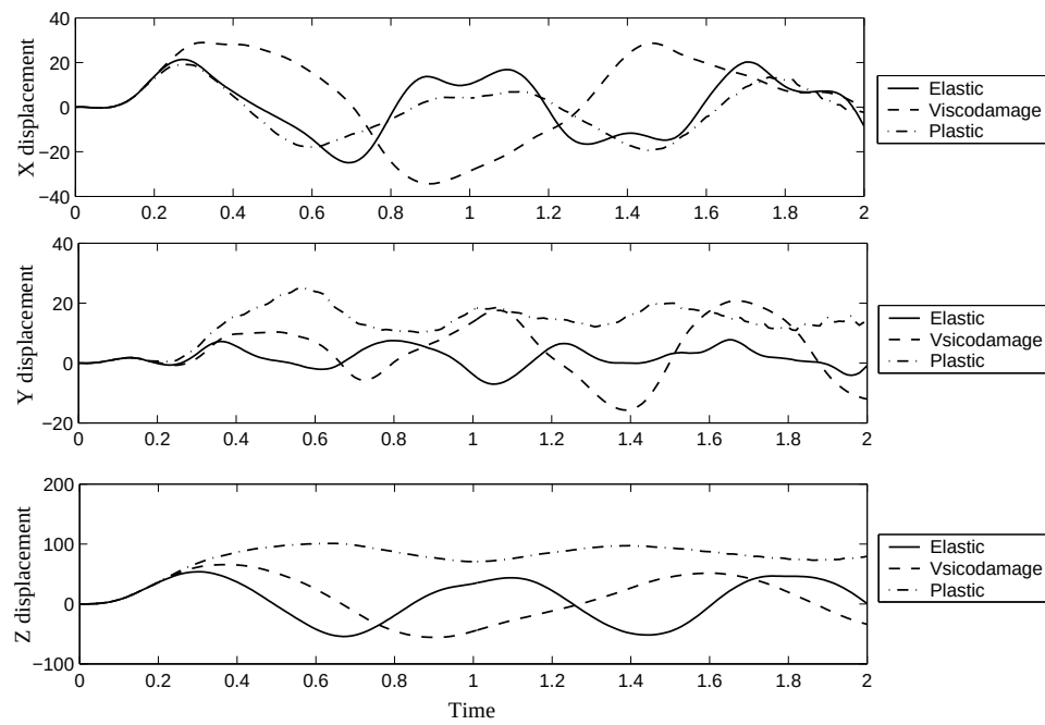
Figure 8.25: Displacement time history response of the node A.
