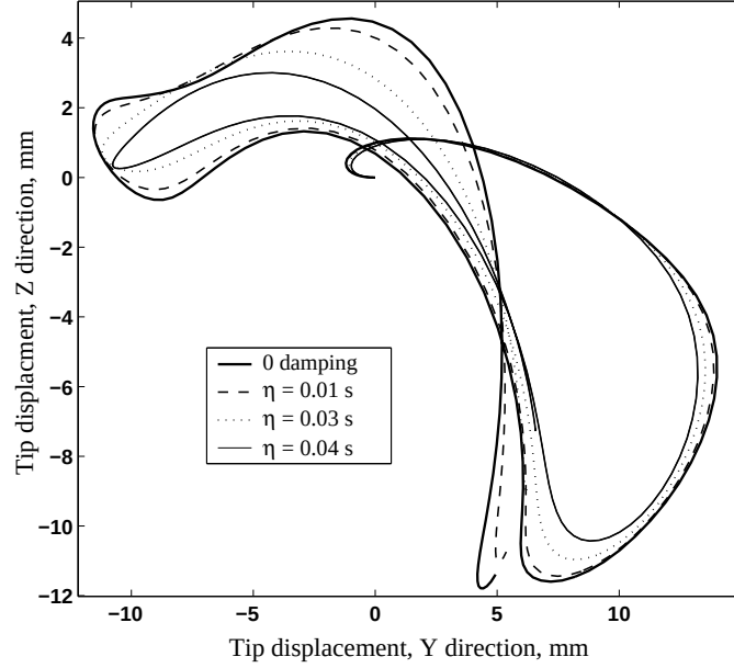
Figure 8.18: Tip displacements time history response in the Y-Z plane.
