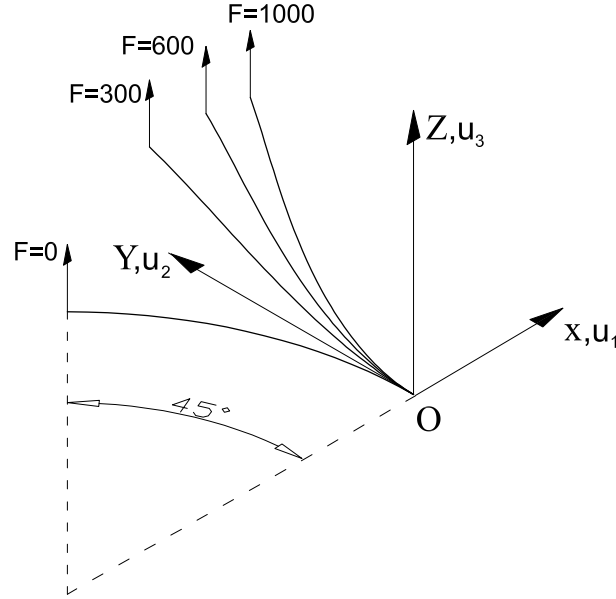
Figure 8.10: Initial geometry and some examples of the deformed configurations for the linear elastic case of the 45^\circ cantilever bend.
