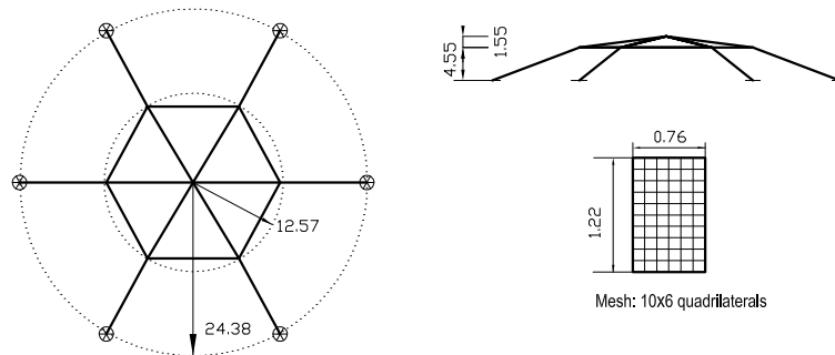
Figure 8.8: Framed dome and detail of the cross sectional mesh.
