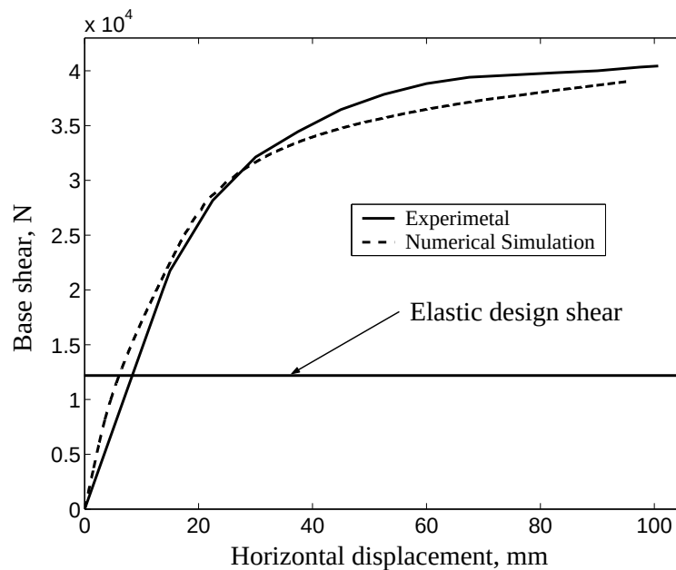
Figure 8.27: Comparison between numerical and experimental push–over analysis: Capacity curves.
