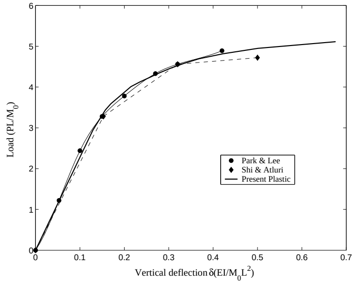
Figure 8.14: Load-deflection curve.
