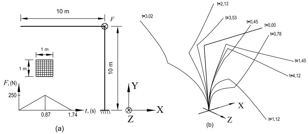
Figure 8.16: Right angle frame. (a): A concentrated out of plane load is applied on the elbow node. (b): Deformed configurations for different time steps for the case of the undamped system.
