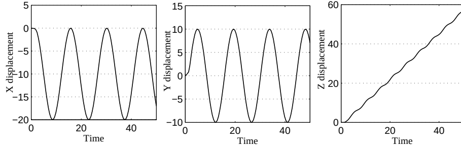
Figure 8.3: Displacements time history response of the free end of the beam.
