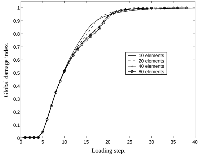
Figure 8.7: Global damage index.
