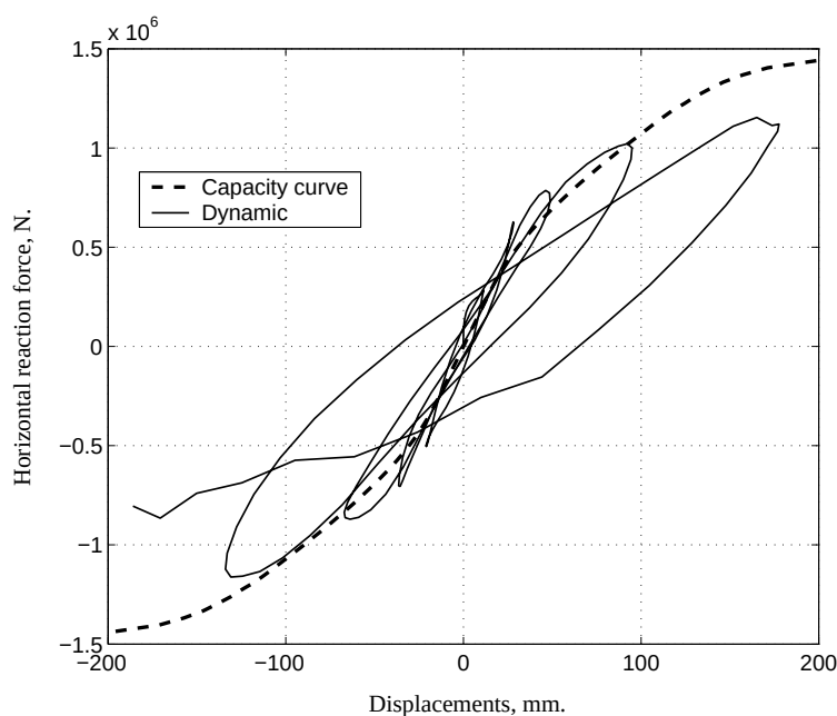
Figure 8.34: Horizontal displacements versus base reaction for the static pushover and the dynamic analysis.
