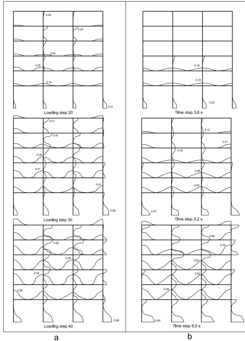
Figure 8.35: Evolution of the local damage indices. (a): Pushover analysis. (b): Dynamic case.
