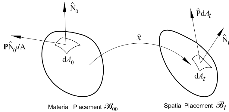
Figure 3.5: Geometric interpretation of the FPK stress tensor; note that \mathbf{P} \cdot \hat{N}_0 dA_0 \in T_{\hat{x}}\mathcal{B}_t although it is drawn on the material placement.
