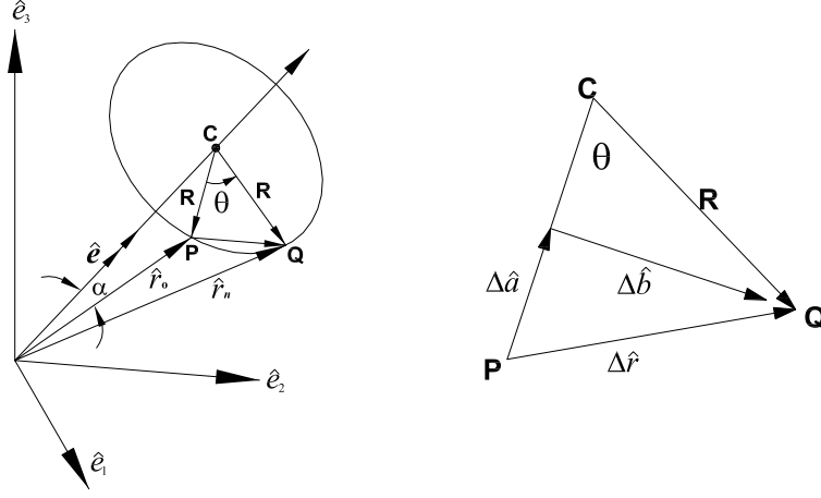
Figure A.3: Rotation vector.
