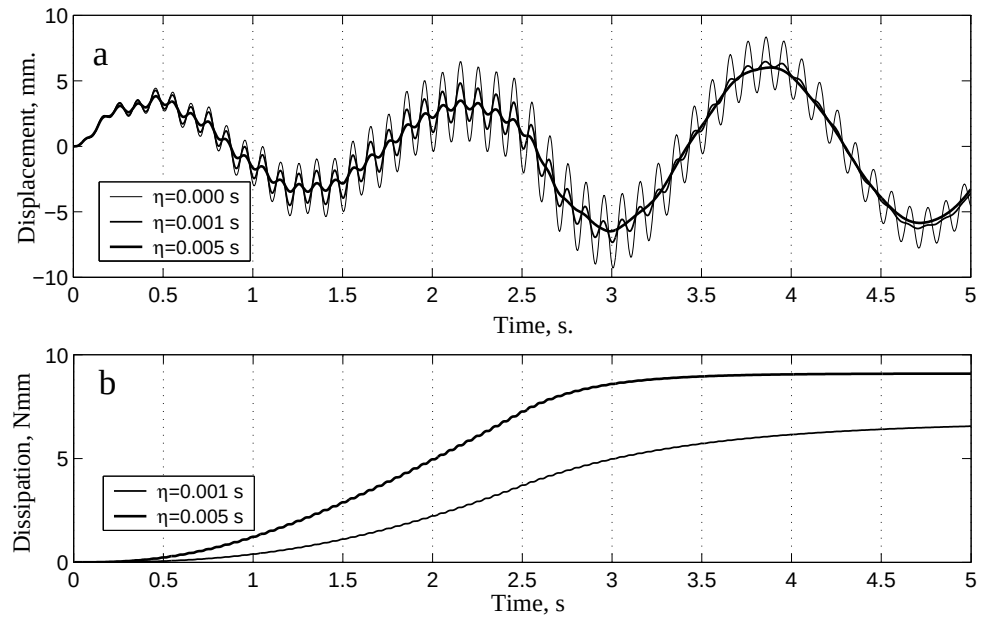
Figure 8.21: (a): High frequency content suppression. (b): Energy dissipation.
