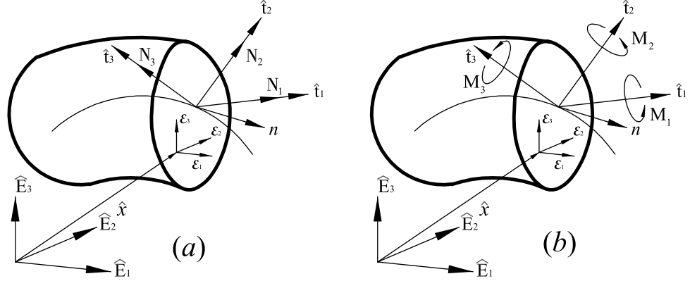
Figure 3.6: Geometric representation of (a): Stress resultant. (b): Stress couple.
