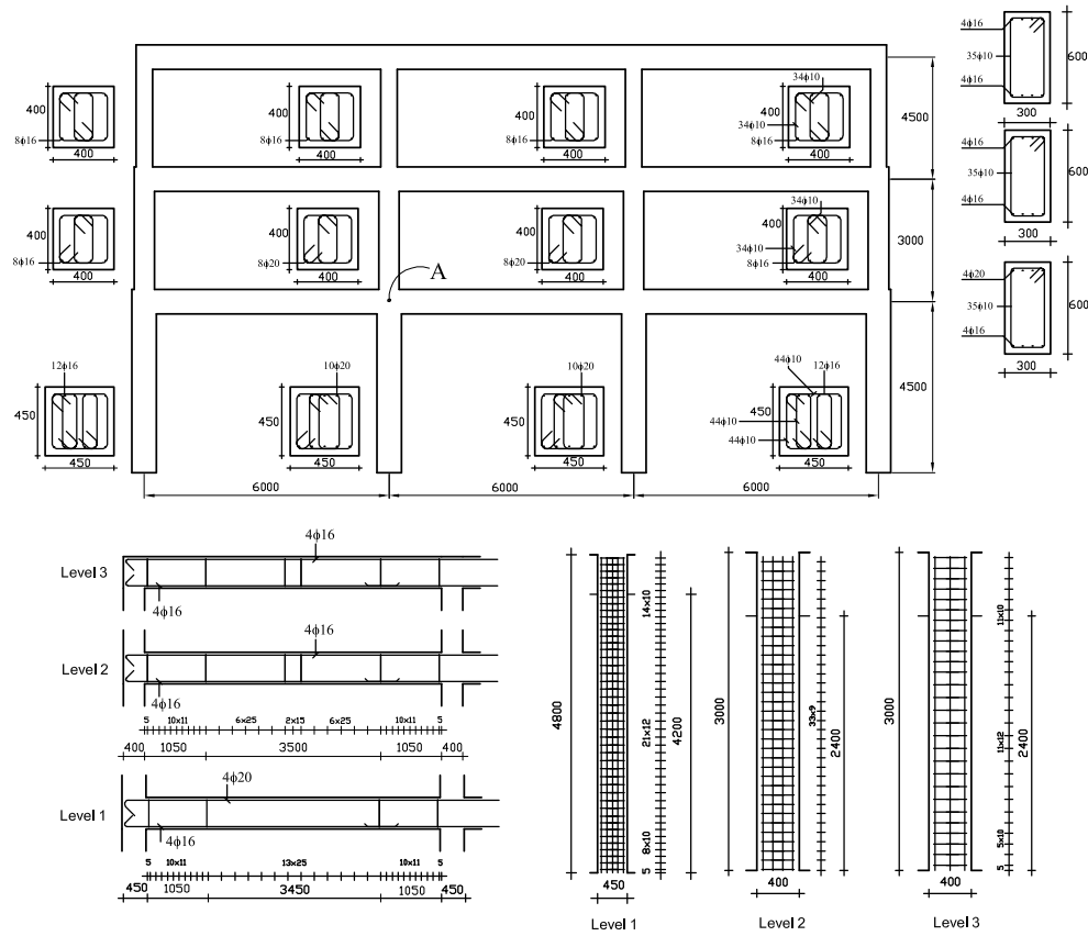
Figure 8.29: RC planar frame details.
