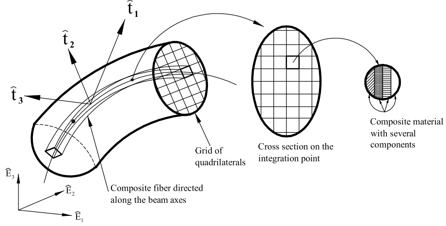
Figure 7.2: Discrete fiber like model of the beam element.
