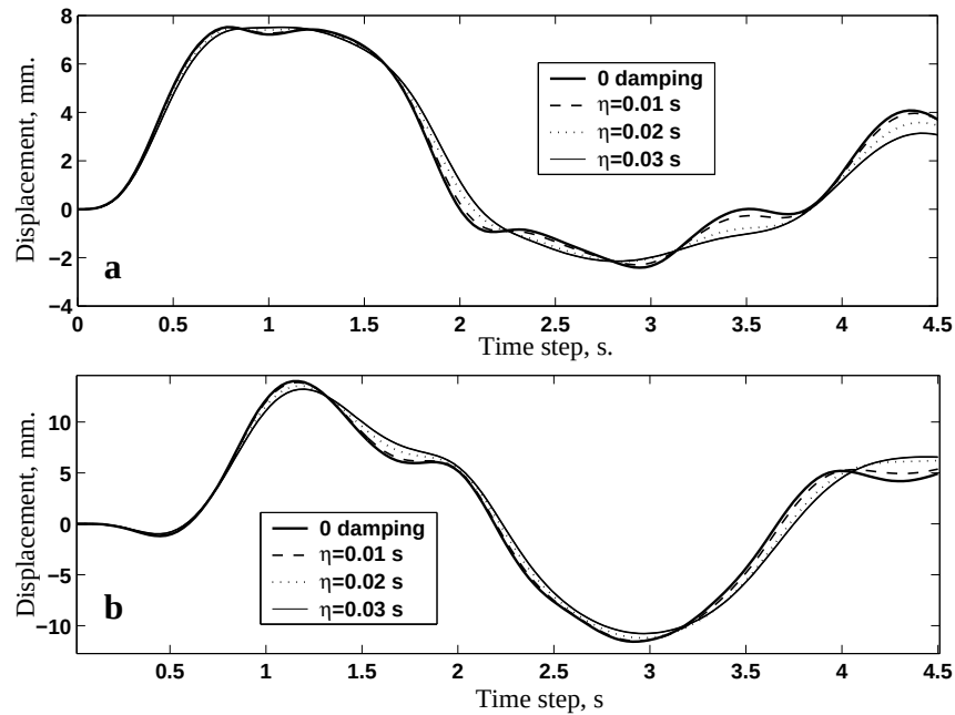
Figure 8.17: Displacement time history responses in the Y direction. (a): Tip. (b): Elbow.
