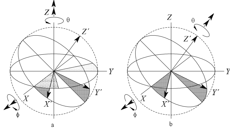
Figure A.2: Composition of rotations in the space. (a): Fixed base: \theta \rightarrow \phi . (b): Movable base: \phi \rightarrow \theta .
