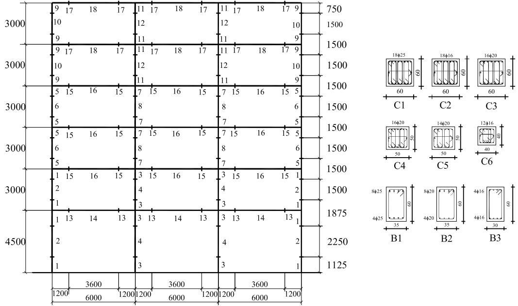
Figure 8.33: Structural model of the RC planar frame.
