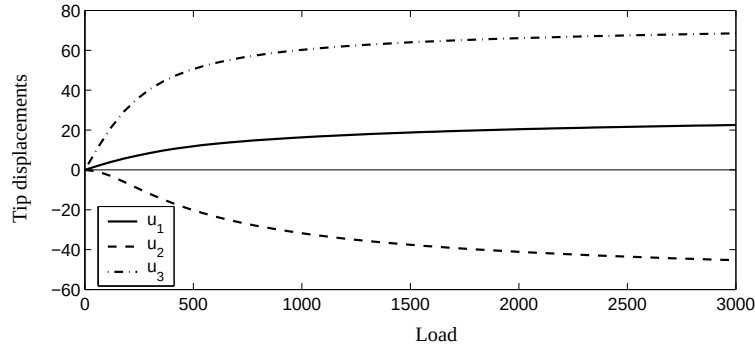
Figure 8.11: Different components of the tip displacement (linear case).
