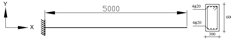
Figure 8.4: RC cantilever beam.
