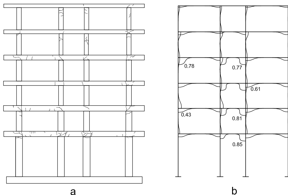
Figure 8.28: Damage. (a): Experimental: Map of fissures. (b): Numerical: Cross sectional damage index.
