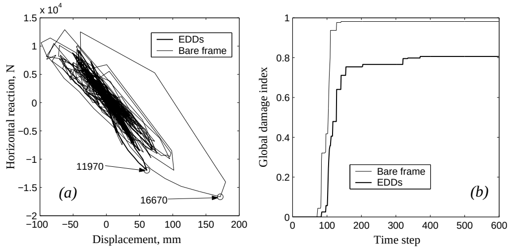
Figure 8.39: (a): Base shear–displacement relationship. (b): Evolution of the global damage index.
