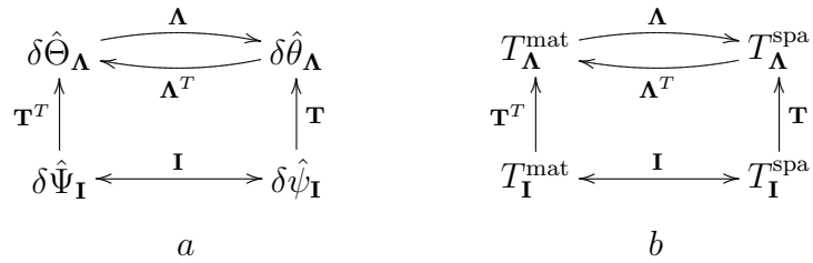
Figure A.9: Commutative diagrams. (a): Configurational description of vectors. (b): Corresponding vector spaces.
