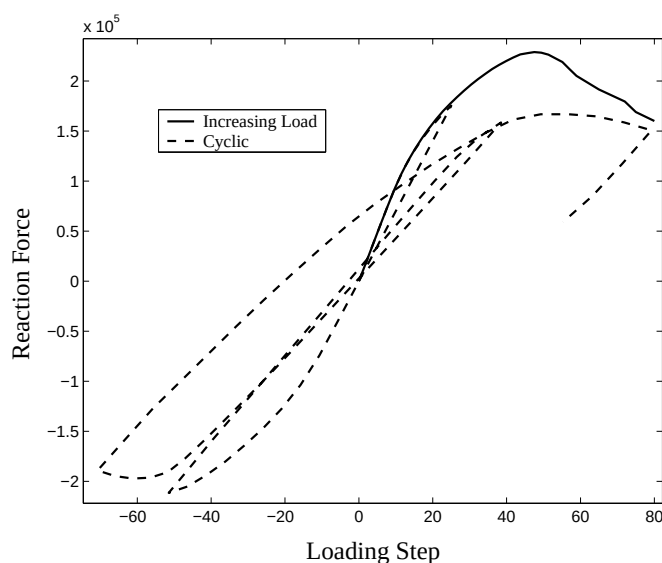
Figure 8.30: Increasing loading versus cyclic loading.
