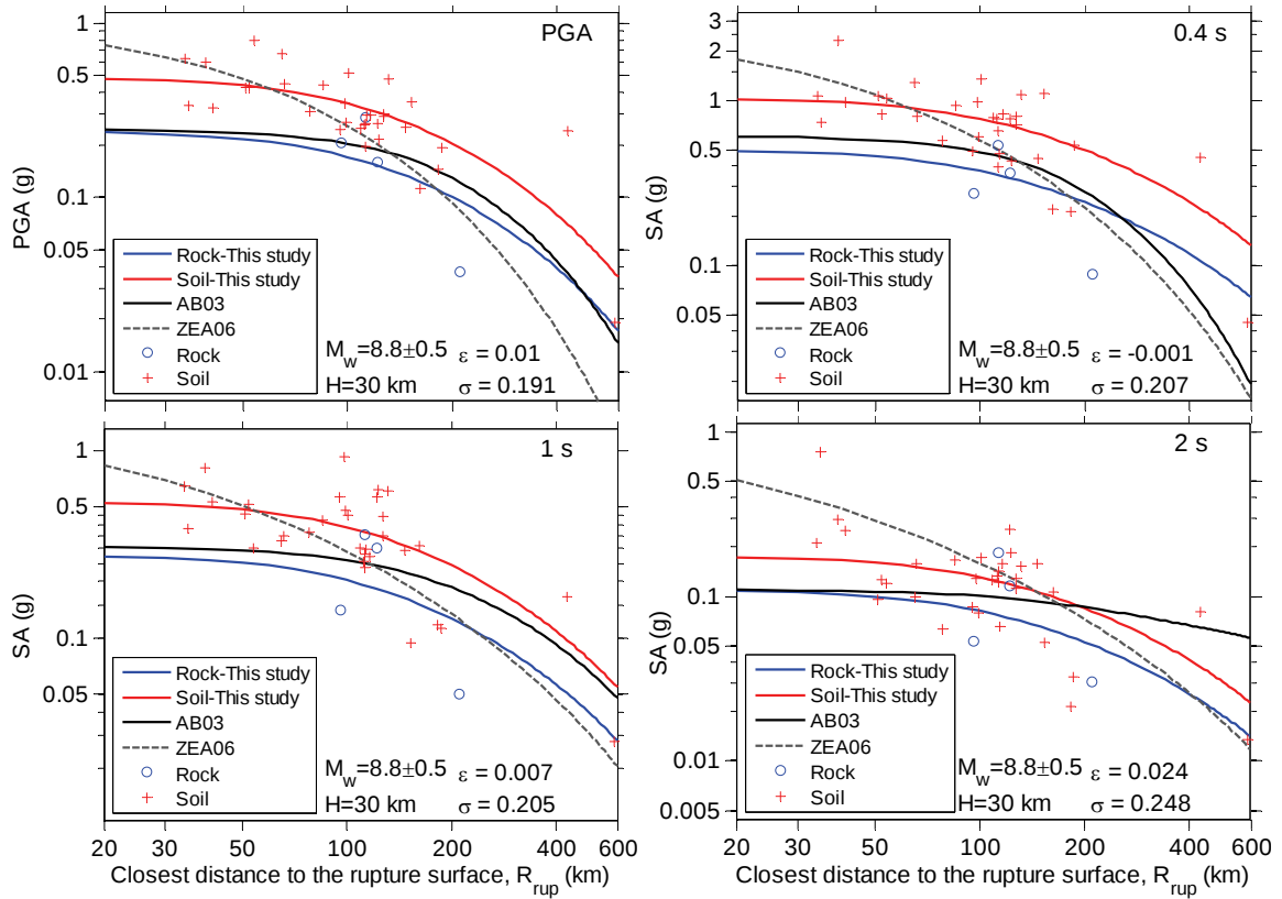
Fig. 8 Comparison between predicted and observed accelerations ( M_w=8.8\pm0.5 , H=30 km). The mean of residuals ( \varepsilon ) and the standard deviation of residuals ( \sigma ) for the data shown are indicated.
