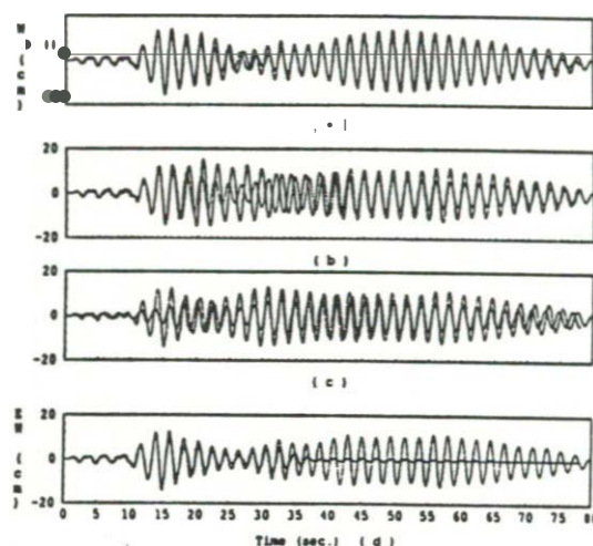
Figure 6: Twelfth floor motion Mt. Lewis event: Input ground motion 0-40 seconds. EW relative displacement, SW corner. a) First three modes, low damping model (1%), b) First mode, low damping model. c) Second mode, low damping model. d) First three modes, moderate damping model (5%). Model — Record .....
